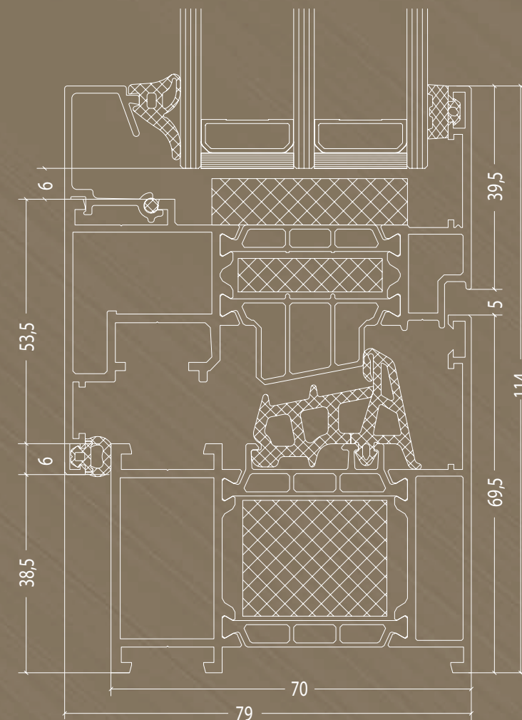
MB-79N SI / WINDOW /
