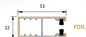
single guide rail
