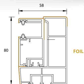
single guide rail
