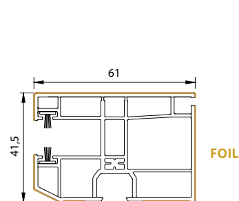
single guide rail
