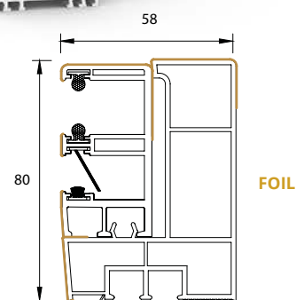
single guide rail with insect screen
