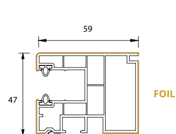
single guide rail
