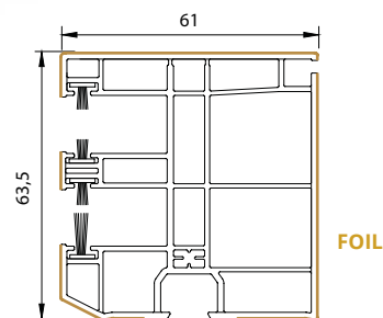
single guide rail with insect screen
