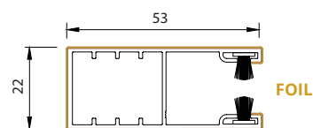
single guide rail
