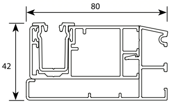
Single guide rail
