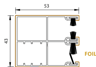
single guide rail with insect screen
