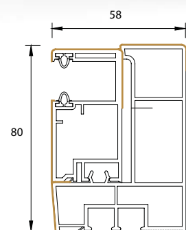
single guide rail
