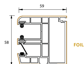
single guide rail with insect screen
