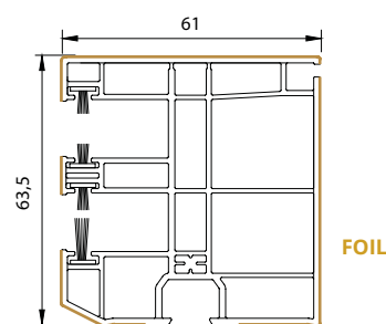
single guide rail with insect screen
