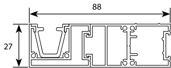
Single guide rail
