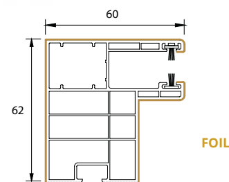
offset guide rail
