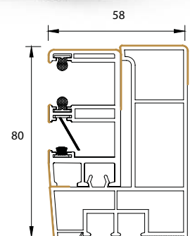
single guide rail with insect screen
