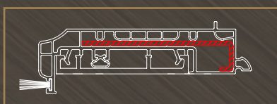
reinforced adapter
